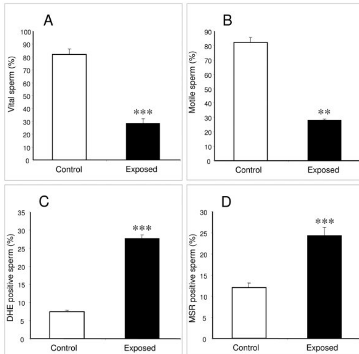
RF-EMR exposure decreases motility and vitality of human sperm while also inducing intracellular ROS. - De Iulius 2009
