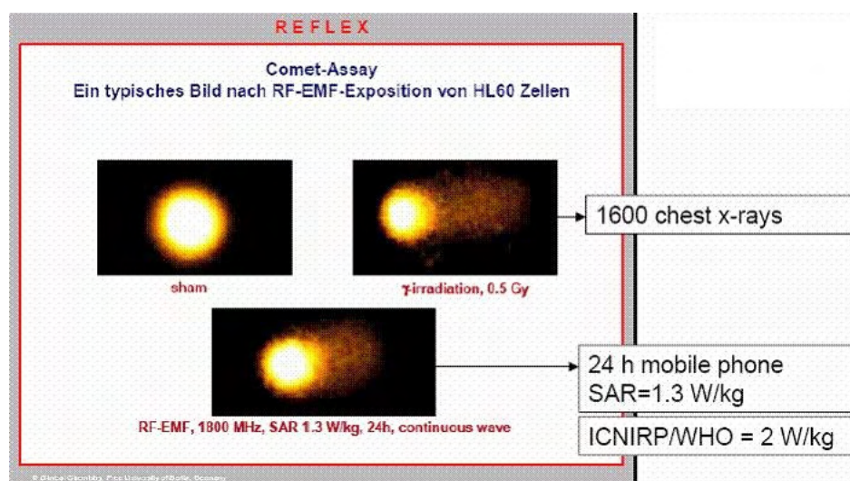
Comparative DNA fragmentation images suggest electromagnetic radiation can produce DNA damage similar to ionising radiation. Reflex 2004
